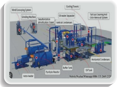
Pyrolysis progress
